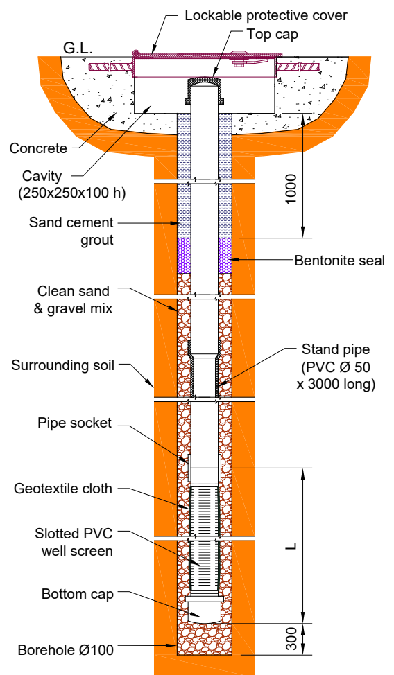
Typical installation scheme of EPP-10SP Open Standpipe
